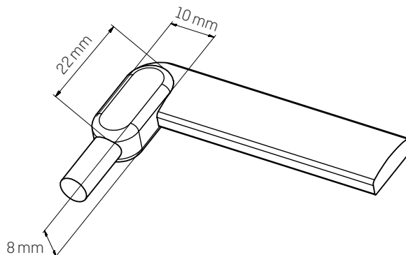
HORIZONTAL CONNECTION
