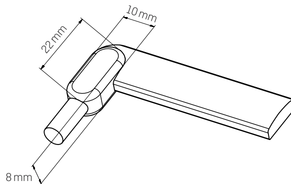
HORIZONTAL CONNECTION
